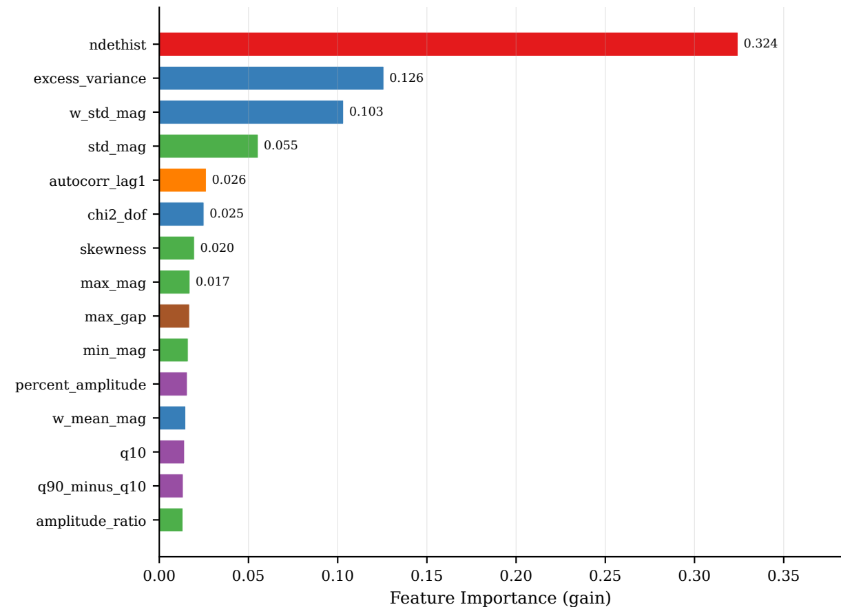
(b) XGBoost-Reduced (39 features, no LS)
