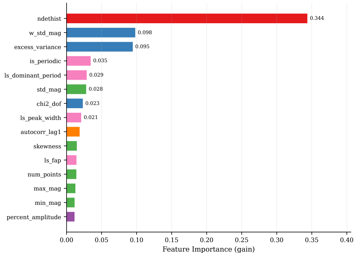
(a) XGBoost-Full (57 features)
